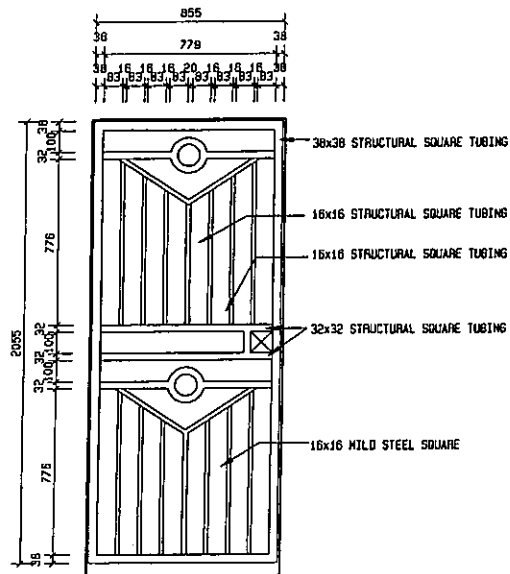
FRONT DOOR GATE 1:25
