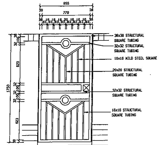
SCREEN WALL GATE 1:25
