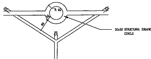
STEEL DETAIL 1:10
