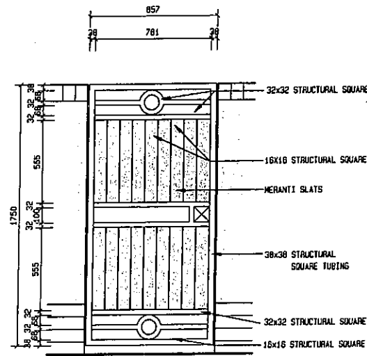
KITCHEN YARD DOOR 1:25
