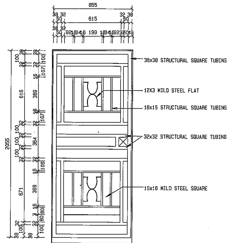
FRONT DOOR GATE 1:25
