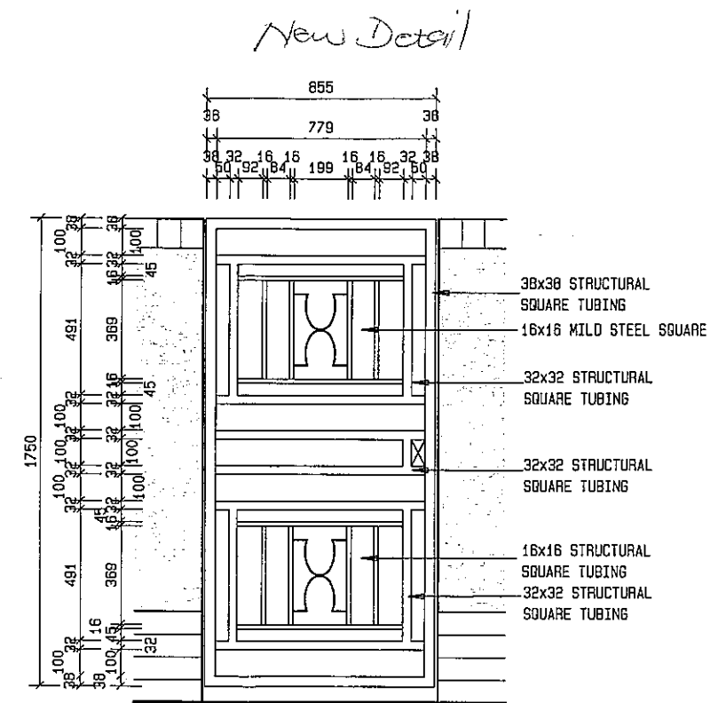
KITCHEN YARD & GARDEN WALL GATE 1:25
