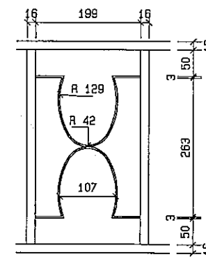
STEEL DETAIL 1:10
